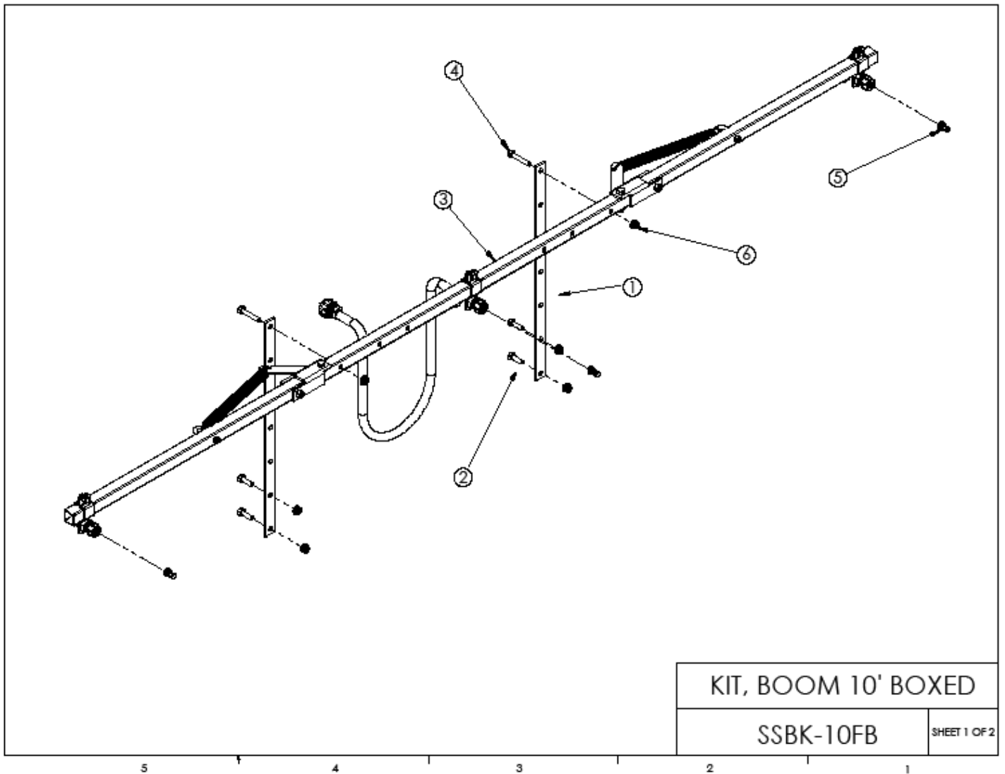
Parts List Figure SSBK-10FB
